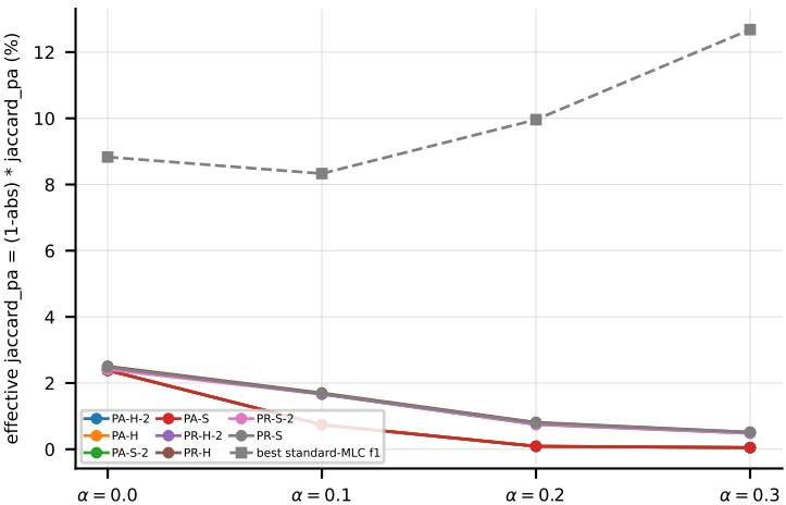
RF on HumanPseAAC (jaccard_pa) -- penalised quality (abstention costs labels)
