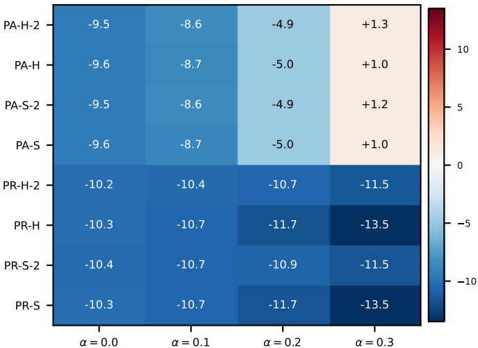
RF on Yeast (jaccard_pa) -- gain (jaccard_pa - f1, percentage points)
