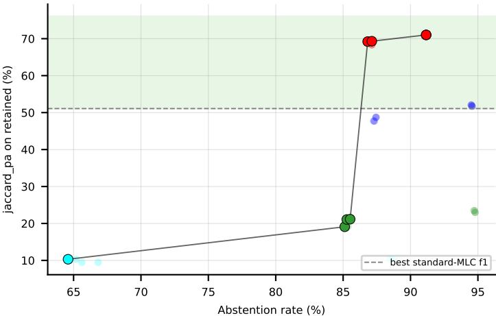
RF on birds (jaccard_pa) -- Pareto frontier + win-region
