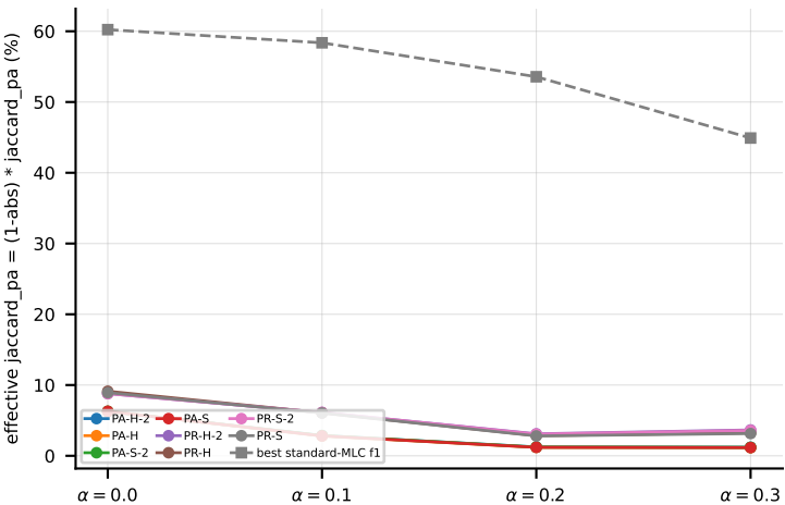
RF on birds (jaccard_pa) -- penalised quality (abstention costs labels)
