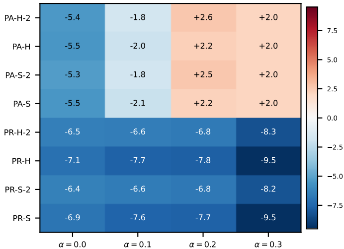
RF on emotions (jaccard_pa) -- gain (jaccard_pa - f1, percentage points)
