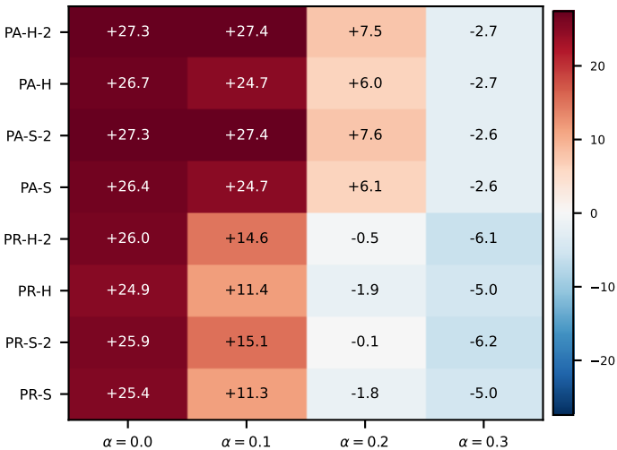
RF on medical (jaccard_pa) -- gain (jaccard_pa - f1, percentage points)
