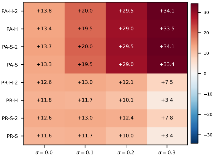
RF on scene (jaccard_pa) -- gain (jaccard_pa - f1, percentage points)
