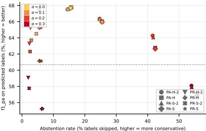
LGBM on Yeast (f1_pa)
