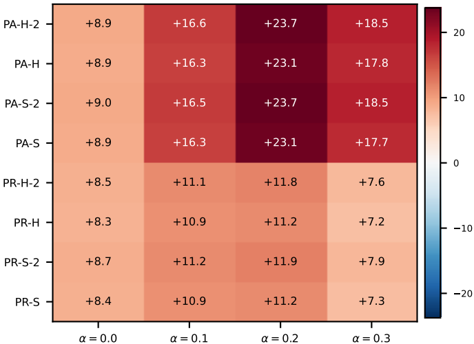
LGBM on scene (f1_pa) -- gain (f1_pa - f1, percentage points)
