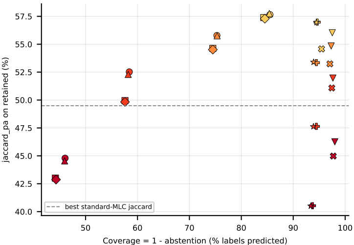
LGBM on Yeast (jaccard_pa) -- robustness: upper-right = robust
