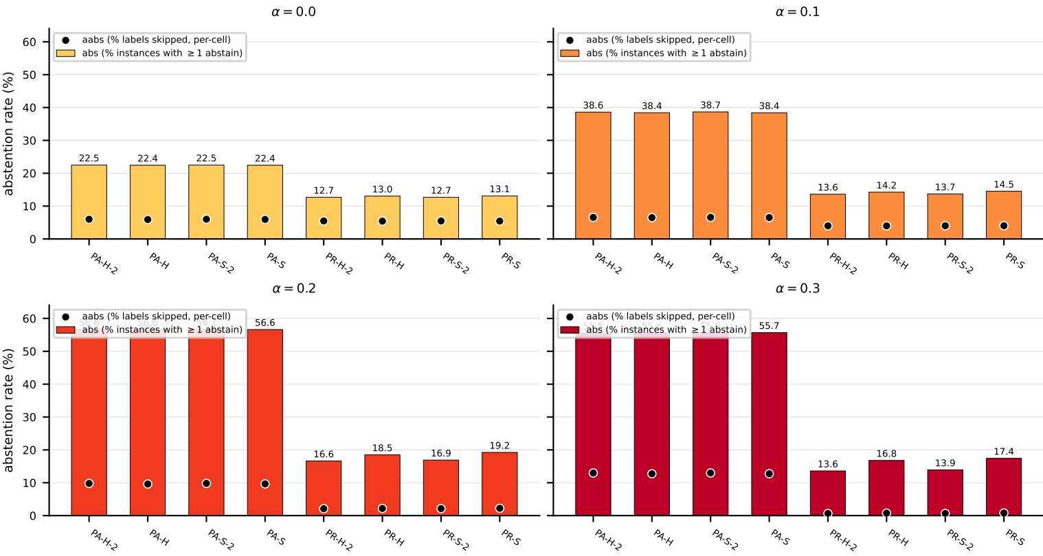
RF on enron: abstention rates
