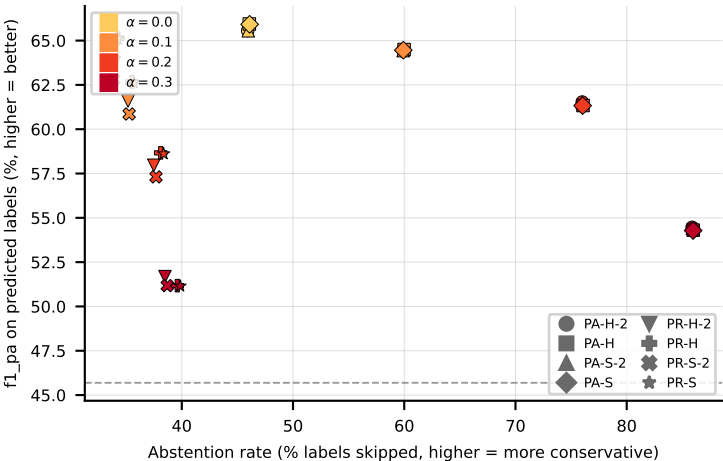
RF aggregate (f1_pa)
