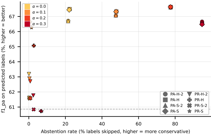
RF on Yeast (f1_pa)
