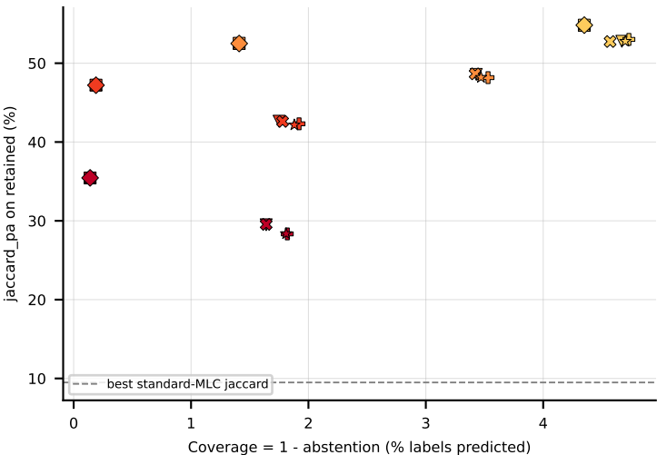
RF on HumanPseAAC (jaccard_pa) -- robustness: upper-right = robust
