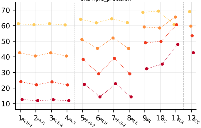
example_precision
