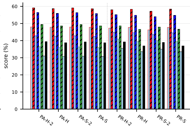
(b) Jaccard paired bars
