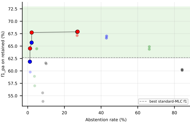
RF on CHD_49 (f1_pa) -- Pareto frontier + win-region
