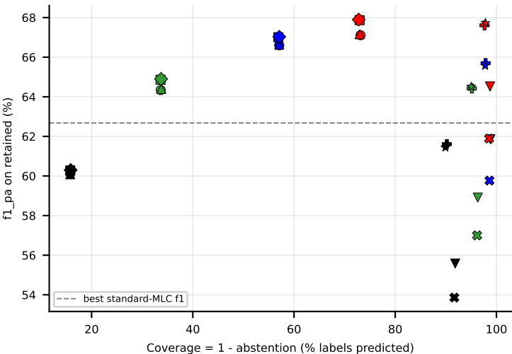
RF on CHD_49 (f1_pa) -- robustness: upper-right = robust
