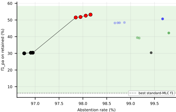
RF on PlantPseAAC (f1_pa) -- Pareto frontier + win-region
