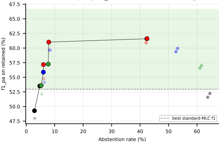
RF on Water-quality (f1_pa) -- Pareto frontier + win-region
