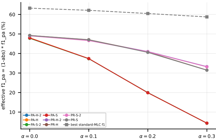
RF on scene (f1_pa) -- penalised quality (abstention costs labels)
