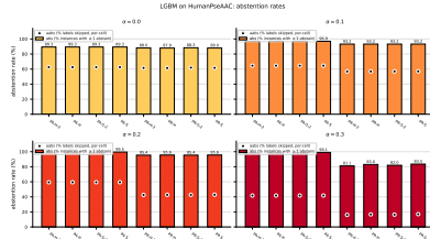
Figure 105: LGBM ( f1_{pa} ) on HumanPseAAC: abstention rates (left) and standard-MLC-vs-abstention paired bars (right), across \alpha \in \{0.0, 0.1, 0.2, 0.3\} . Left: bar = \text{abs} (% of instances with at least one abstained label, instance-level); dot = \text{aabs} (% of labels skipped, per-cell label-level). These rates are independent of the quality metric. Right: blue = standard MLC quality (no abstention) on the matched BV metric; coloured = with-abstention quality on retained labels.
