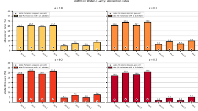
Figure 117: LGBM (f1_pa) on Water-quality: abstention rates (left) and standard-MLC-vs-abstention paired bars (right), across \alpha \in \{0.0, 0.1, 0.2, 0.3\} . Left: bar = abs (% of instances with at least one abstained label, instance-level); dot = aabs (% of labels skipped, per-cell label-level). These rates are independent of the quality metric. Right: blue = standard MLC quality (no abstention) on the matched BV metric; coloured = with-abstention quality on retained labels.
