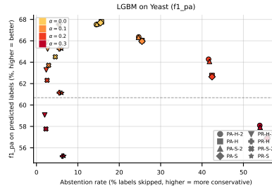
Figure 110: LGBM ( f1_{pa} ) on Yeast : coverage-risk scatter. Each point is one (method, noise) pair; x = abstention rate, y = quality on retained labels. Points above the dashed line beat the best standard-MLC baseline.
