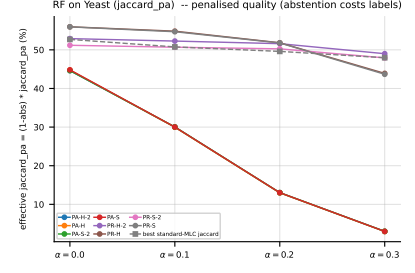
Figure 72: RF (jaccard_pa) on Yeast — robustness view. Left: efficiency-quality scatter ( x = \text{coverage} = 1 - \text{abs} ); upper-right is robust (predicts many labels and keeps quality high). Right: effective jaccard_pa = (1 - \text{abs}) \cdot \text{jaccard\_pa} , i.e. retained quality penalised by skipped coverage. A method whose effective curve stays above the dashed standard-MLC baseline at every \alpha is robust to noise, not just selectively abstaining on hard labels.
