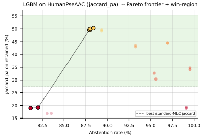
Figure 143: LGBM (jaccard_pa) on HumanPseAAC: Pareto frontier of (abstention, retained quality) with the win-region shaded green (left); per-method per-noise gain ( \text{jaccard\_pa} - f_1 ) heatmap (right).
