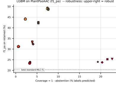
Figure 104: LGBM ( f1_{pa} ) on PlantPseAAC — robustness view. Left: efficiency-quality scatter ( x = coverage = 1 - \text{abs} ); upper-right is robust (predicts many labels and keeps quality high). Right: effective f1_{pa} = (1 - \text{abs}) \cdot f1_{pa} , i.e. retained quality penalised by skipped coverage. A method whose effective curve stays above the dashed standard-MLC baseline at every \alpha is robust to noise, not just selectively abstaining on hard labels.
