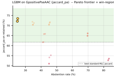
Figure 127: LGBM (jaccard_pa) on GpositivePseAAC : Pareto frontier of (abstention, retained quality) with the win-region shaded green (left); per-method per-noise gain ( \text{jaccard\_pa} - f_1 ) heatmap (right).
