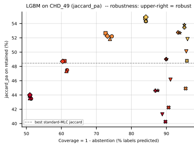
Figure 152: LGBM (jaccard_pa) on CHD_49 — robustness view. Left: efficiency-quality scatter ( x = \text{coverage} = 1 - \text{abs} ); upper-right is robust (predicts many labels and keeps quality high). Right: effective jaccard\_pa = (1 - \text{abs}) \cdot jaccard\_pa , i.e. retained quality penalised by skipped coverage. A method whose effective curve stays above the dashed standard-MLC baseline at every \alpha is robust to noise, not just selectively abstaining on hard labels.
