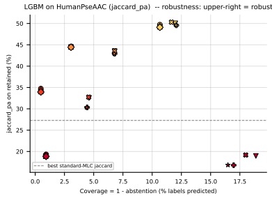
Figure 144: LGBM (jaccard_pa) on HumanPseAAC — robustness view. Left: efficiency-quality scatter ( x = \text{coverage} = 1 - \text{abs} ); upper-right is robust (predicts many labels and keeps quality high). Right: effective jaccard_pa = (1 - \text{abs}) \cdot \text{jaccard\_pa} , i.e. retained quality penalised by skipped coverage. A method whose effective curve stays above the dashed standard-MLC baseline at every \alpha is robust to noise, not just selectively abstaining on hard labels.
