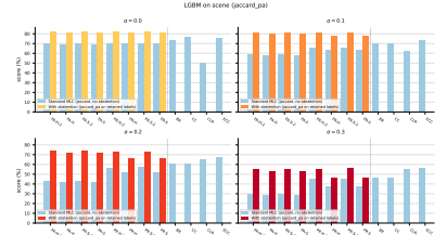
Figure 133: LGBM ( \text{jaccard\_pa} ) on scene : abstention rates (left) and standard-MLC-vs-abstention paired bars (right), across \alpha \in \{0.0, 0.1, 0.2, 0.3\} . Left: bar = \text{abs} (% of instances with at least one abstained label, instance-level); dot = \text{aabs} (% of labels skipped, per-cell label-level). These rates are independent of the quality metric. Right: blue = standard MLC quality (no abstention) on the matched BV metric; coloured = with-abstention quality on retained labels.
