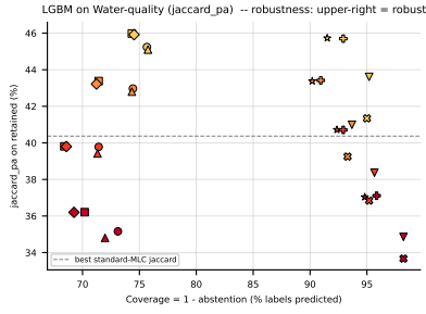
Figure 156: LGBM ( \text{jaccard\_pa} ) on Water-quality — robustness view. Left: efficiency-quality scatter ( x = \text{coverage} = 1 - \text{abs} ); upper-right is robust (predicts many labels and keeps quality high). Right: effective \text{jaccard\_pa} = (1 - \text{abs}) \cdot \text{jaccard\_pa} , i.e. retained quality penalised by skipped coverage. A method whose effective curve stays above the dashed standard-MLC baseline at every \alpha is robust to noise, not just selectively abstaining on hard labels.
