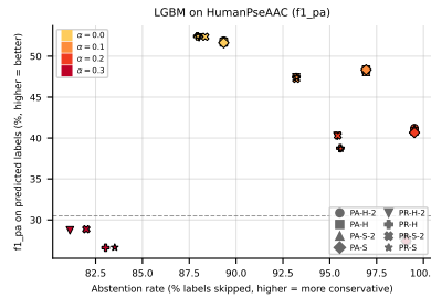
Figure 106: LGBM ( f1_{pa} ) on HumanPseAAC: coverage-risk scatter. Each point is one (method, noise) pair; x = abstention rate, y = quality on retained labels. Points above the dashed line beat the best standard-MLC baseline.
