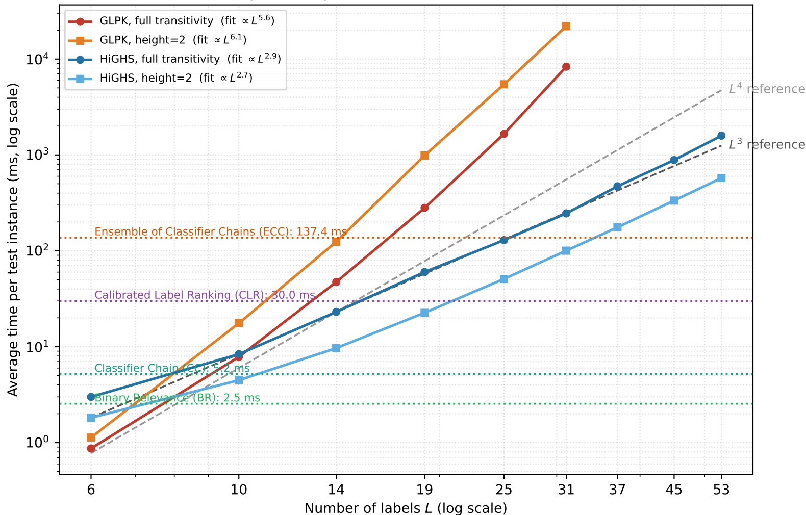
Per-instance ILP runtime scaling -- Subset (0/1 exact-match) accuracy (real enron RF pairwise probabilities, mean over 300 test instances)
