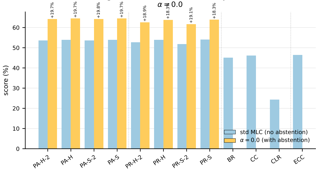
RF averaged across all datasets — f_1 paired bars
