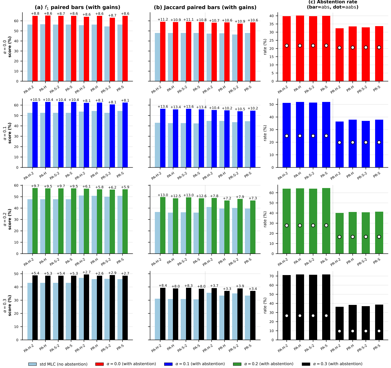
Figure 4: LGBM averaged across all datasets, 4×3 grid (rows = \alpha , cols = f_1 / Jaccard / abstention rate) — (version 2) only the 8 PA/PR methods that can abstain; gain labels + x.y printed above each with-abstention bar so the score-point benefit over the std-MLC bar at the same method is visible at a glance. Same colour / layout conventions as version 1. Color = \alpha \in \{0.0, 0.1, 0.2, 0.3\} .
