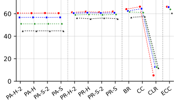
micro- f_1 (??) ( \uparrow )
