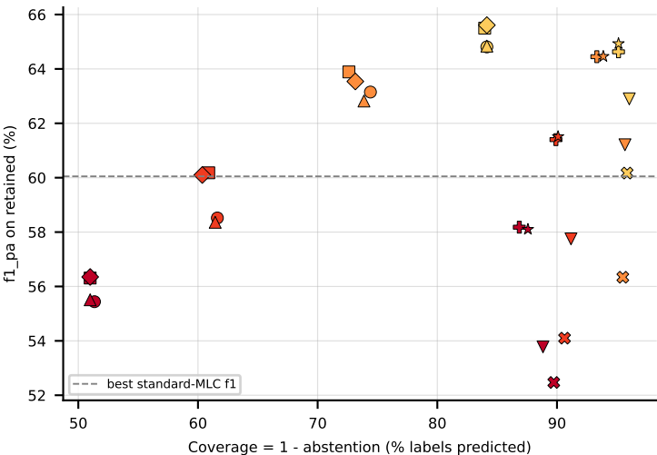
LGBM on CHD_49 (f1_pa) -- robustness: upper-right = robust
