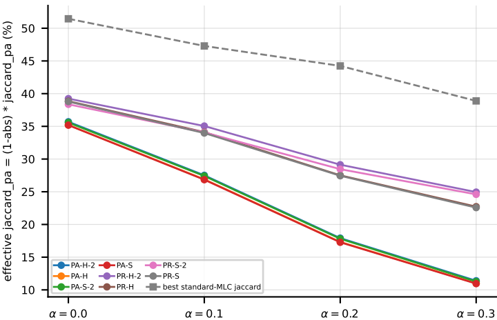
LGBM aggregate (jaccard_pa) -- penalised quality (abstention costs labels)
