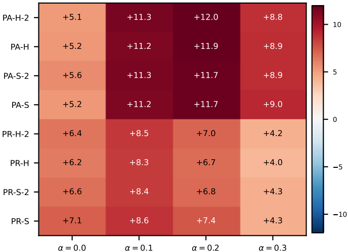
RF on VirusPseAAC (f1_pa) -- gain (f1_pa - f1, percentage points)
