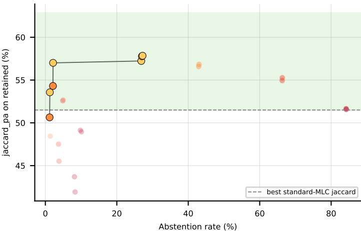
RF on CHD_49 (jaccard_pa) -- Pareto frontier + win-region
