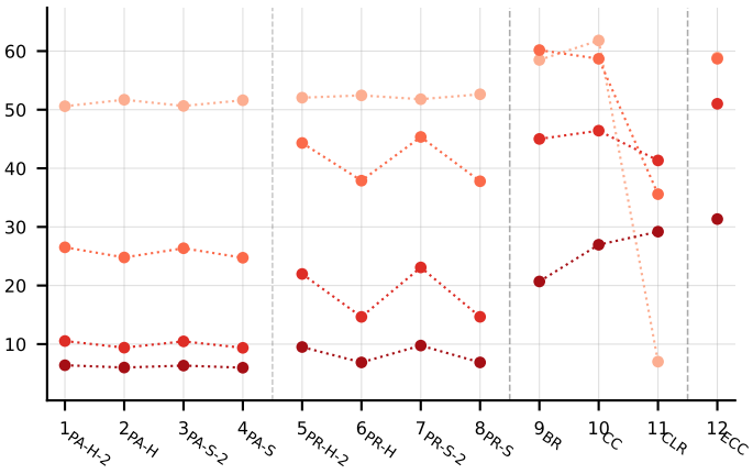
jaccard
