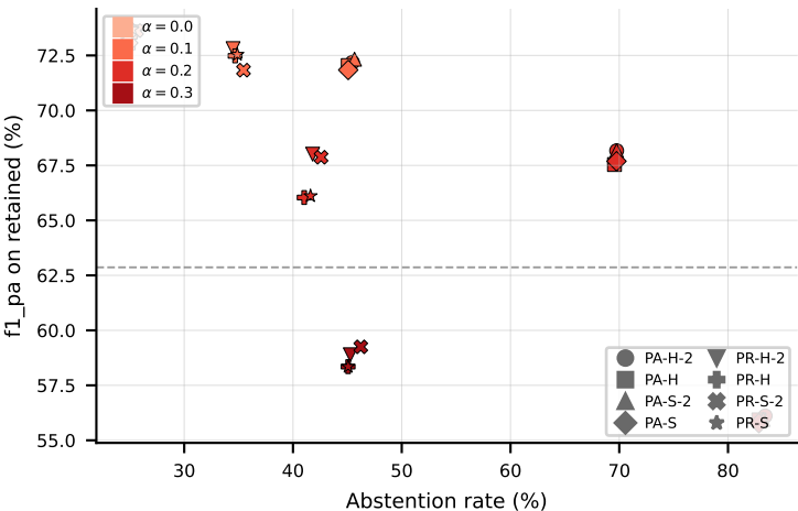
LGBM on GpositivePseAAC
