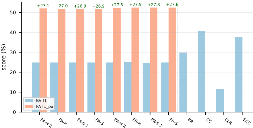
LGBM on HumanPseAAC ( \alpha = 0.0 )
