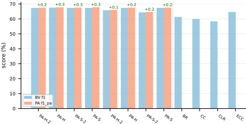
LGBM on Yeast ( \alpha = 0.0 )
