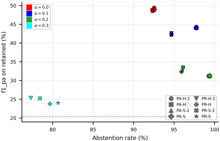
LGBM on PlantPseAAC
