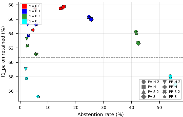
LGBM on Yeast
