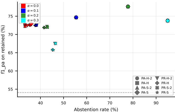
RF on GpositivePseAAC
