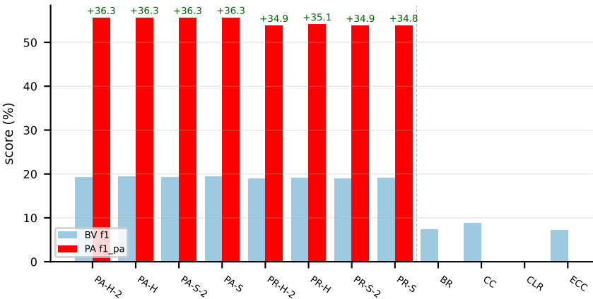
RF on HumanPseAAC ( \alpha = 0.0 )
