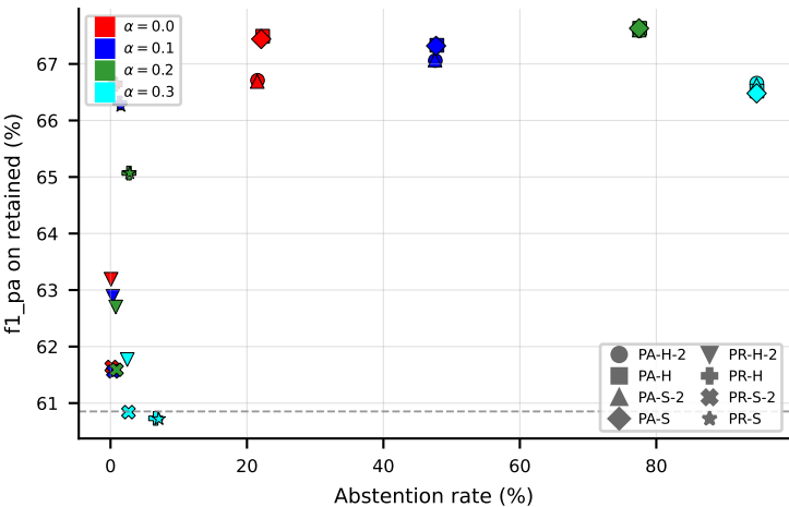
RF on Yeast
