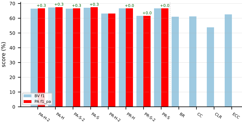
RF on Yeast ( \alpha = 0.0 )
