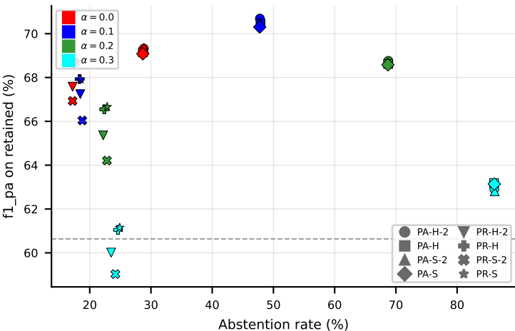
RF on emotions
