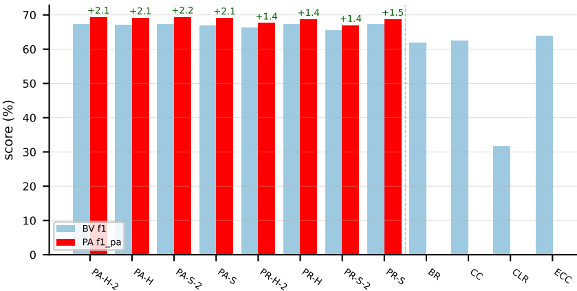
RF on emotions ( \alpha = 0.0 )
