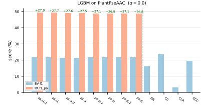
Figure 15: LGBM on PlantPseAAC: coverage-risk (left) and BV-vs-PA paired bars (right).
