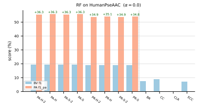
Figure 6: RF on HumanPseAAC: coverage-risk (left) and BV-vs-PA paired bars (right).
