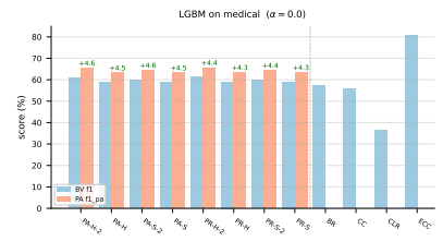
Figure 19: LGBM on medical: coverage-risk (left) and BV-vs-PA paired bars (right).
