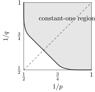
FIGURE 1. The exact constant-one region for quadratic output on the binary cube. The curved pieces correspond to flat-biased one-dimensional extremizers; the central straight pieces lie on the full-cube line.
