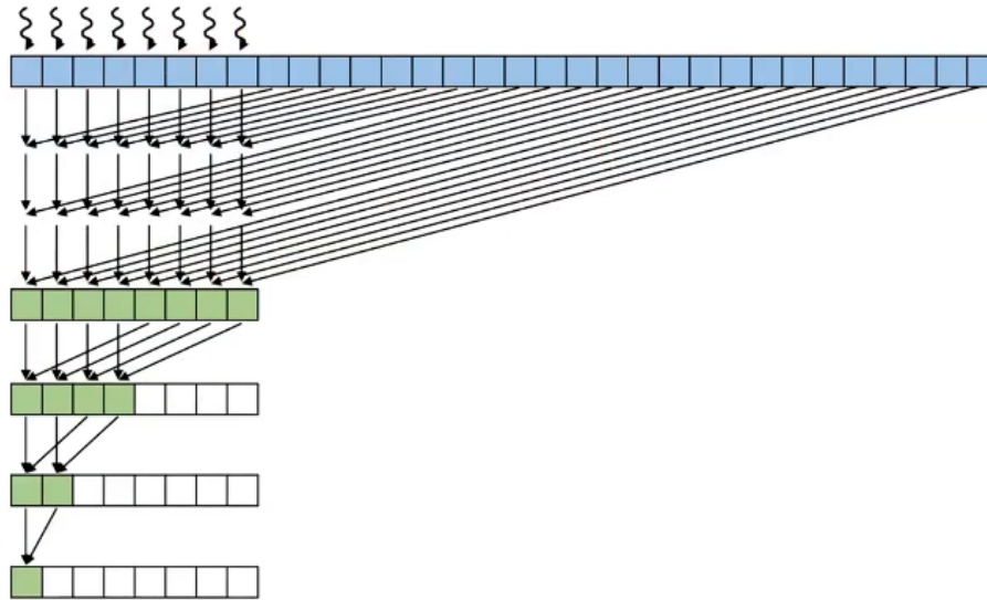
Figure 3: thread coarsening
