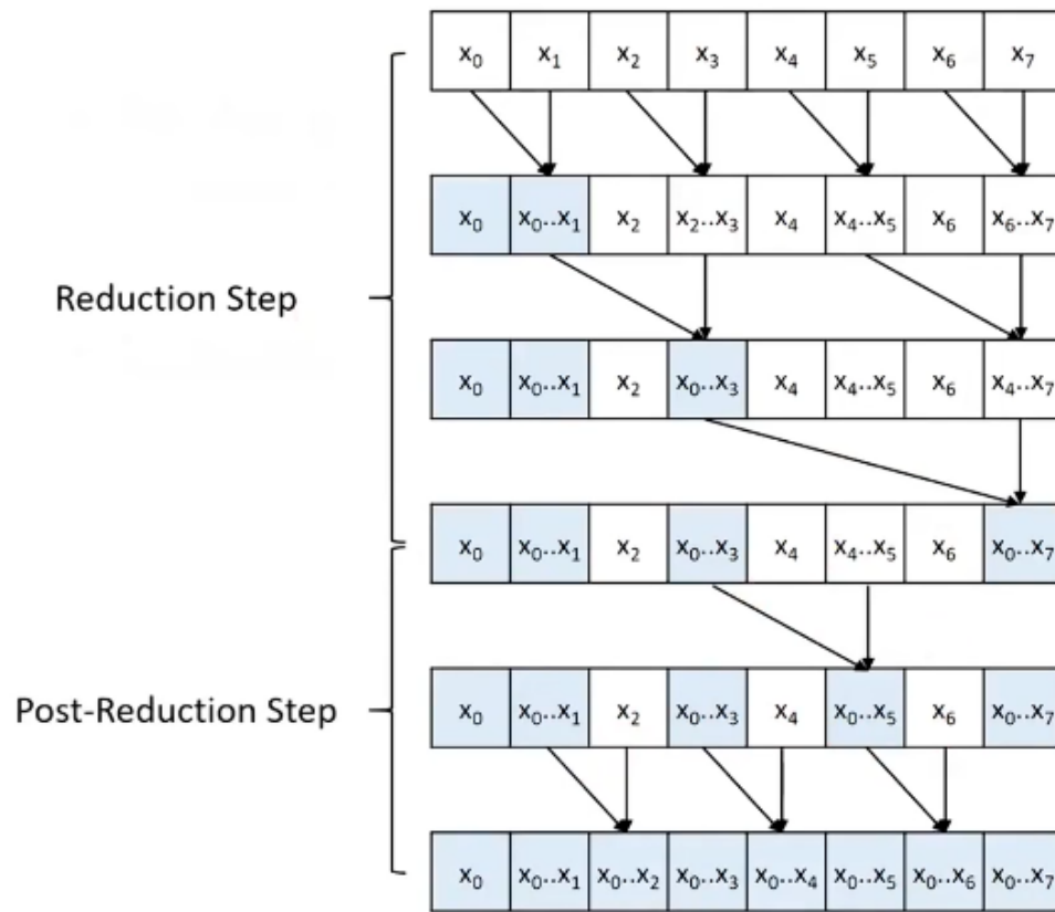
Figure 6: Brent-Kung Parallel (Inclusive) Scan
