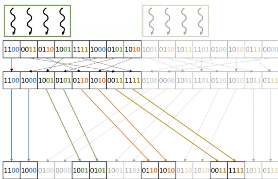
Figure 12: Radix Sort with Thread Coarsening
