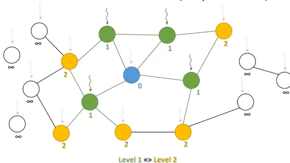
Figure 19: Vertex-Centric BFS (Top-Down)
