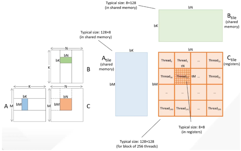
Figure 27: Use Large Tiles
