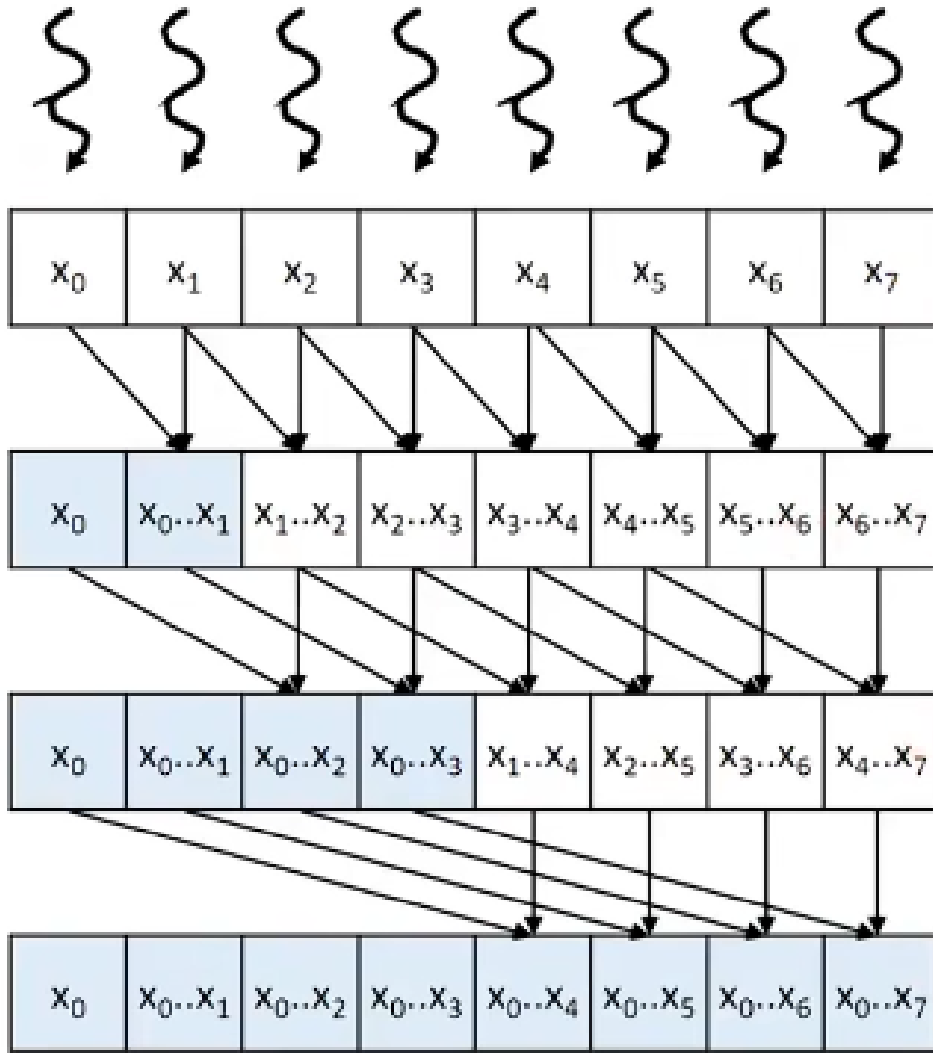
Figure 5: Kogge-Stone parallel (inclusive) scan
