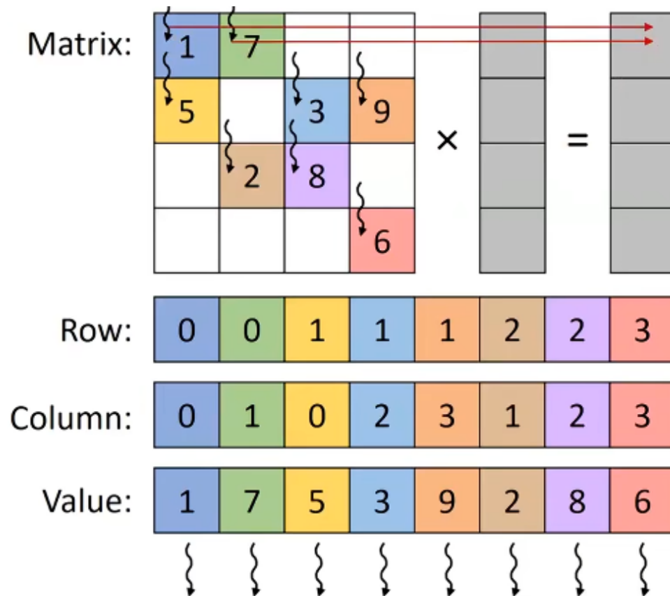
Figure 14: SpMV/COO
