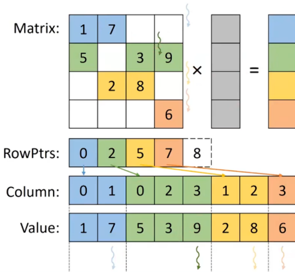
Figure 15: SpMV/CSR
