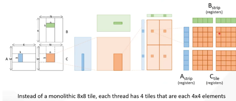
Figure 30: Rearranging Tiles to Coalesce Stores
