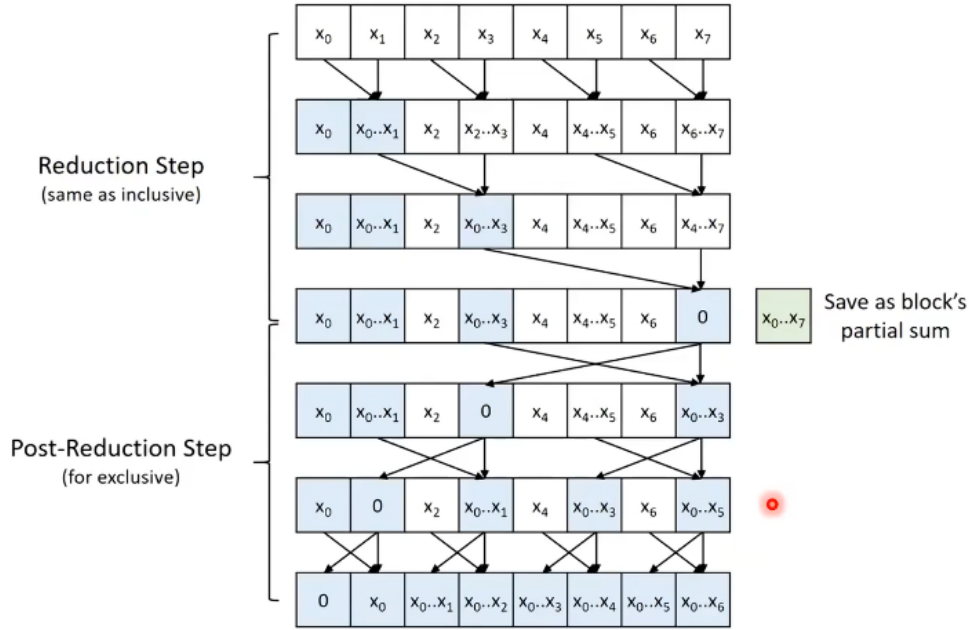
Figure 7: Brent-Kung Parallel (Exclusive) Scan
