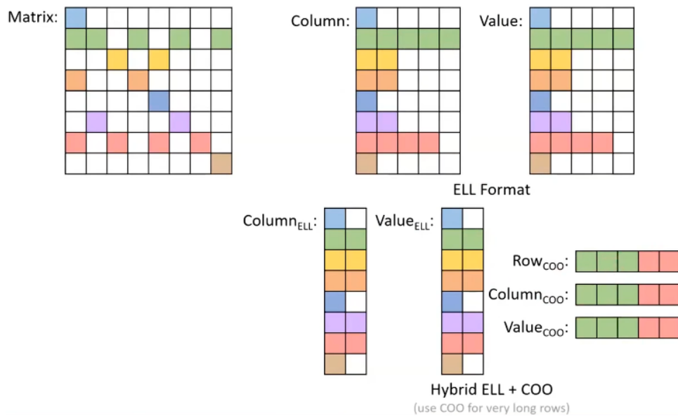
Figure 17: Hybrid ELL COO
