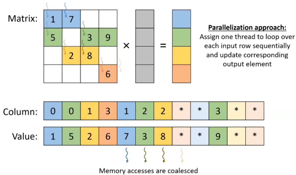
Figure 16: SpMV ELL
