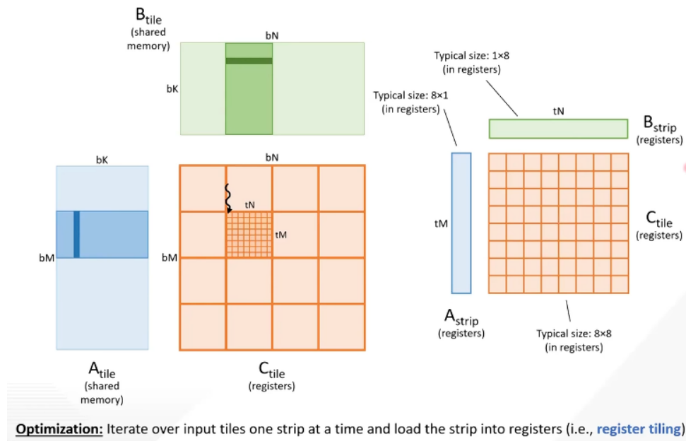
Figure 29: Register Tiling
