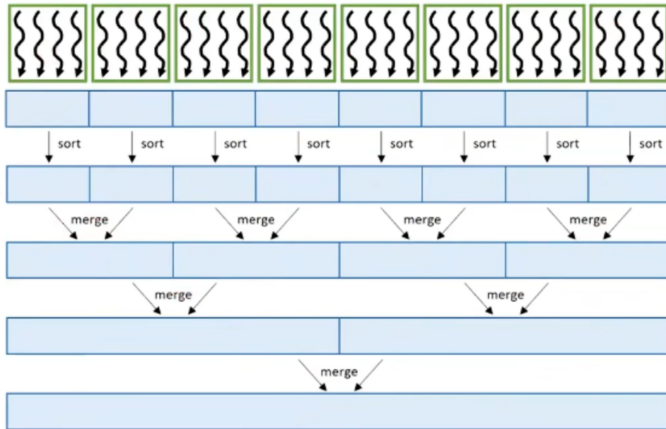
Figure 13: Merge Sort
