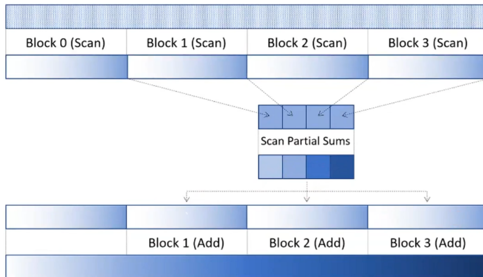
Figure 4: segmented scan
