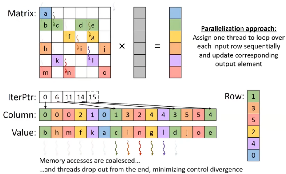
Figure 18: SpMV JDS Kernel
