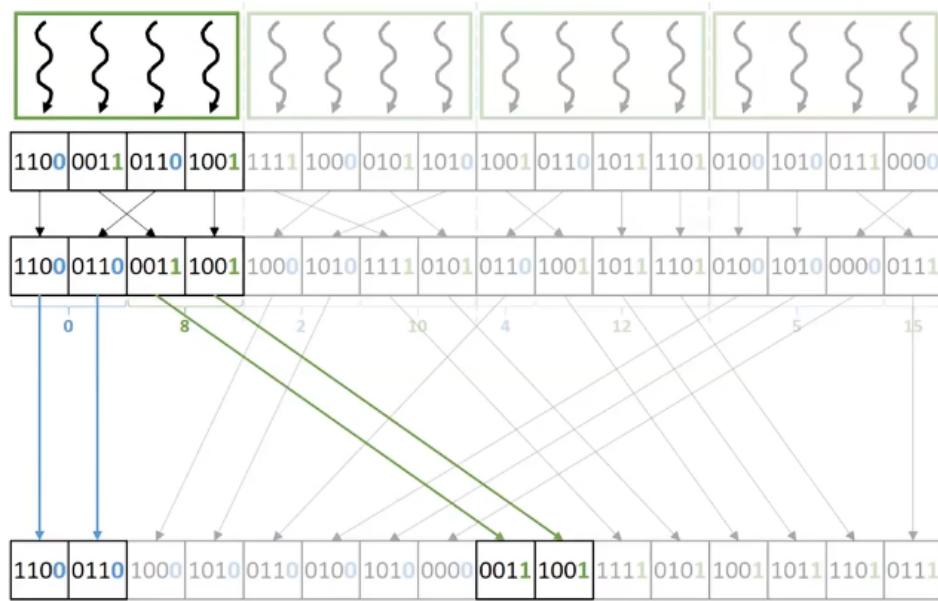
Figure 11: optimizing memory coalescing
