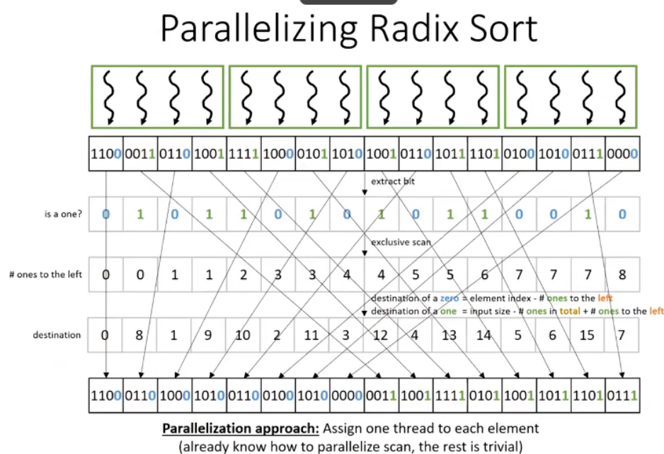
Figure 10: paralleling radix sort
