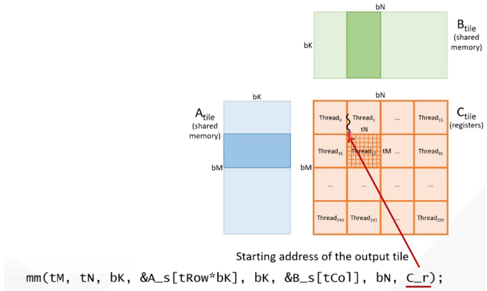
Figure 28: Computing Thread Tile
