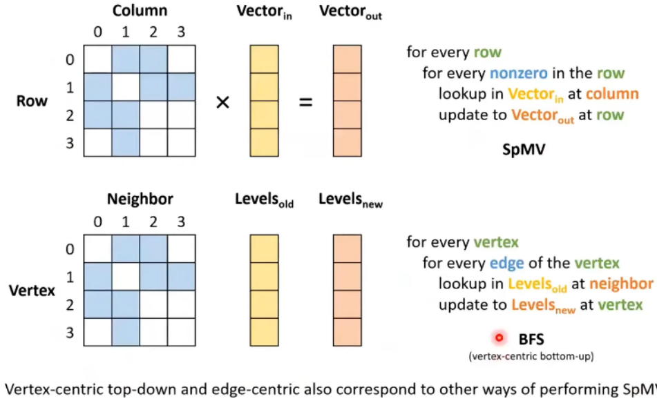
Figure 22: Similarity between BFS and SpMV
