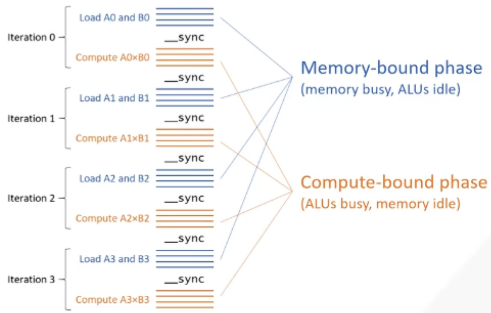
Figure 31: Motivation for Software Pipelining
