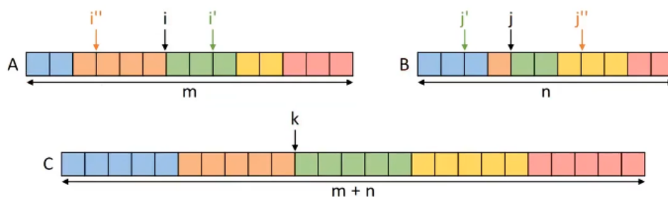
Figure 8: Finding Input Segments
