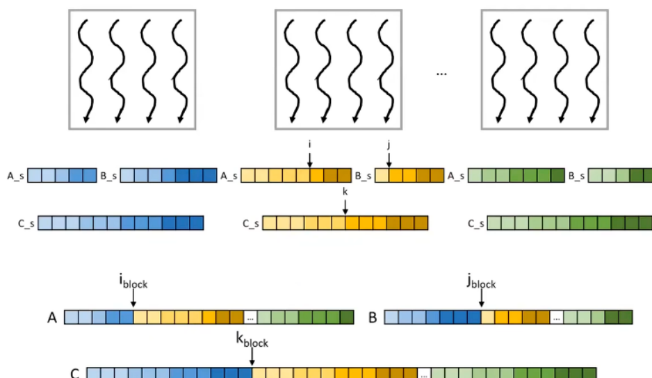
Figure 9: Shared Memory Tiling
