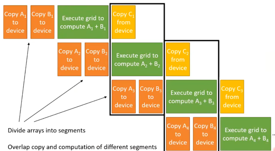
Figure 25: Pipelining Vector Addition
