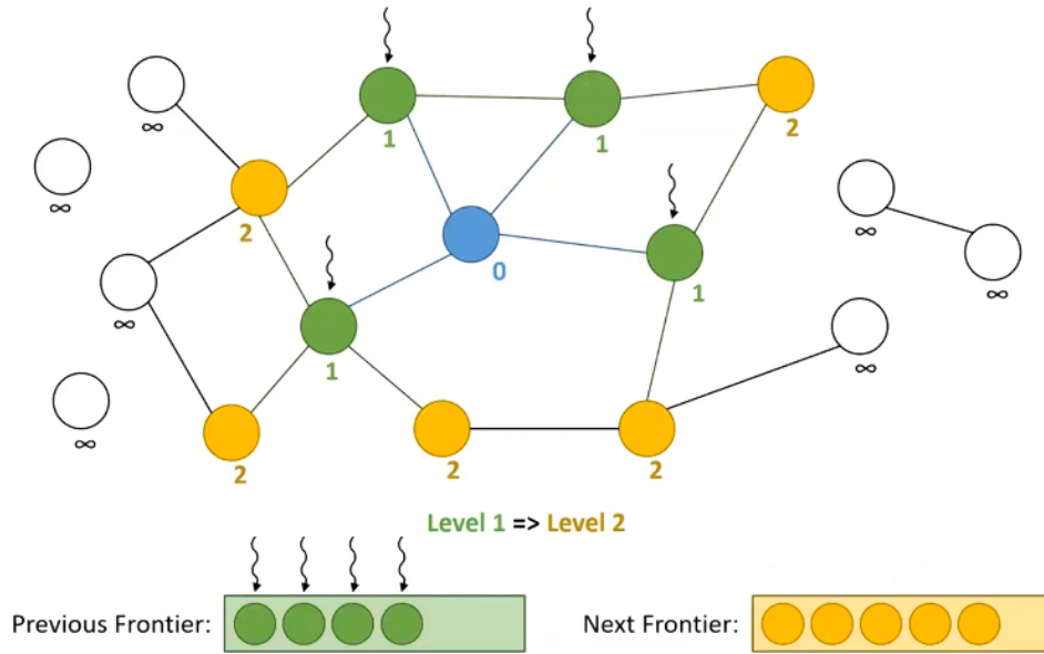
Figure 23: Vertex-Centric Frontier-Based BFS
