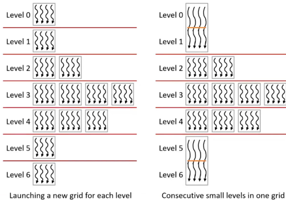
Figure 24: Minimizing Launch Overhead
