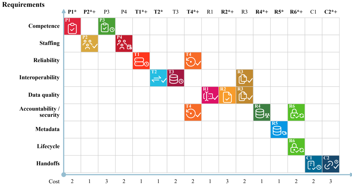
Figure 2: Coverage of requirements by candidate indicators
