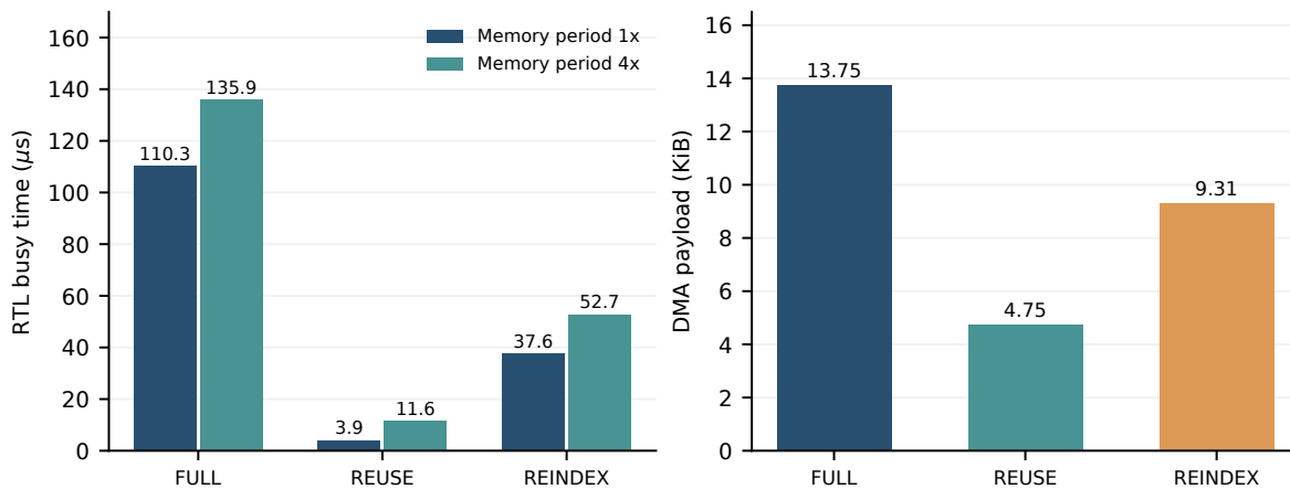
Fig. 6. Measured H32/N64/K8 command latency with two online memory periods, and DMA payload (identical across periods). REUSE preserves an earlier selection; REINDEX evaluates a supplied subset. These different workloads are not interchangeable accuracy baselines. Payload includes result and gathered-KV writes, excluding host uploads, MMIO, readback, and link framing.
