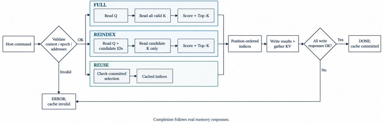
Fig. 4. Accepted START lifecycle. Candidate blocks are expanded externally. REUSE bypasses scoring; DONE waits for all write responses. Failures invalidate the cache, while an illegal doorbell is rejected before START.
