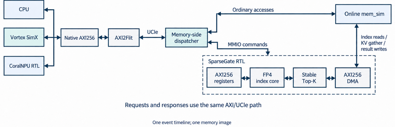
Fig. 1. System placement. Vortex command-processor DMA sends the gate’s AXI register requests; CPU and CoralNPU remain ordinary traffic sources on the shared link. SparseGate is after UClc; ordinary accesses retain a bypass. The C++ memory-side dispatcher is a verification adapter, while the register endpoint, score/selection core, and DMA are synthesizable RTL. Return data and completion follow the original protocol path. Conceptual illustration; exact protocol contracts are in the artifact.
