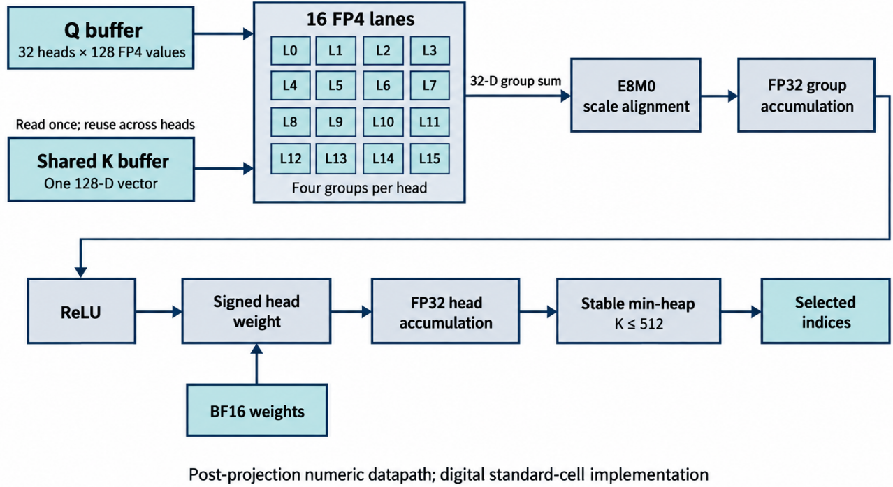
Post-projection numeric datapath; digital standard-cell implementation
