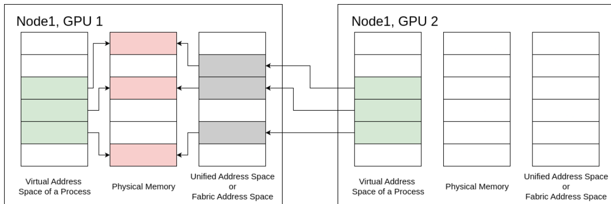
Figure 53: Unicast Memory Sharing Example
