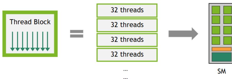
Figure 19: A thread block is partitioned into warps of 32 threads.
