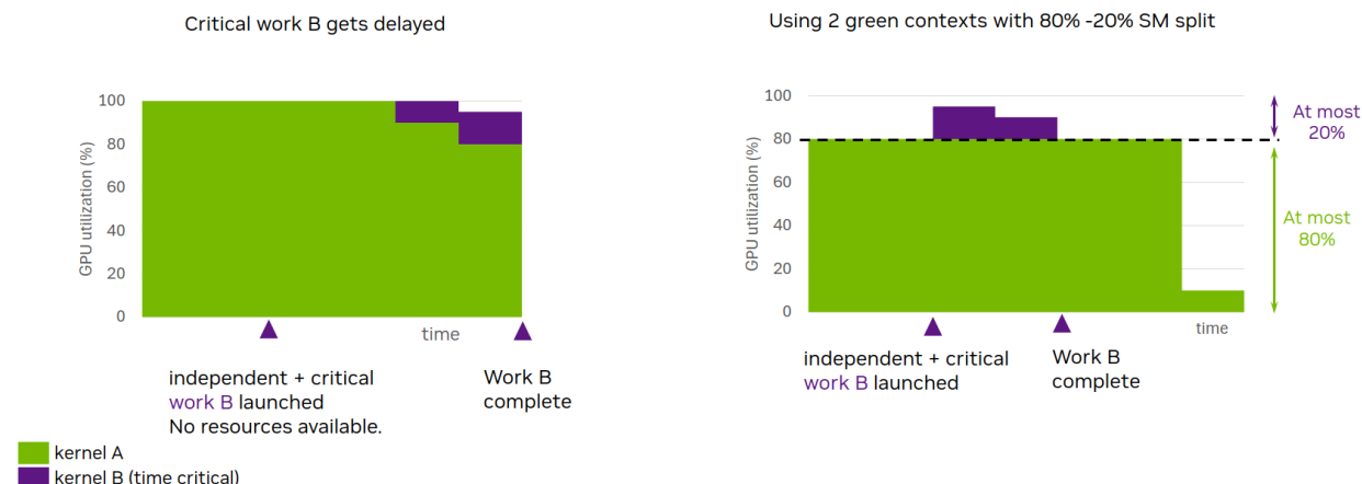
Figure 42: Motivation: GCs' static resource partitioning enables latency-sensitive work B to start and complete sooner
