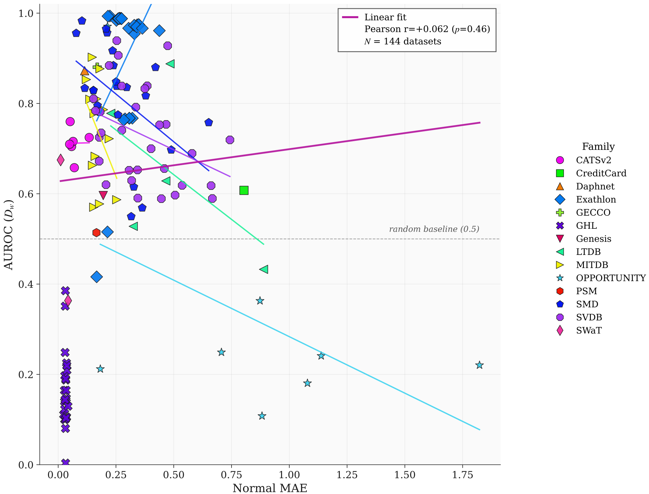
Forecast MAE vs anomaly-detection AUROC ( N = 144 datasets)
