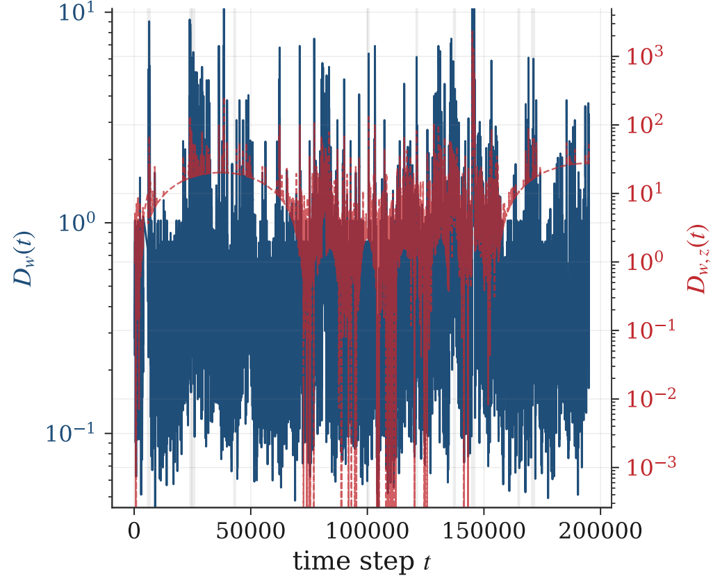
(b) Median: CATSv2_id_2 \text{AUROC}_{D_w} = 0.725 , \text{AUROC}_{D_{w,z}} = 0.681
