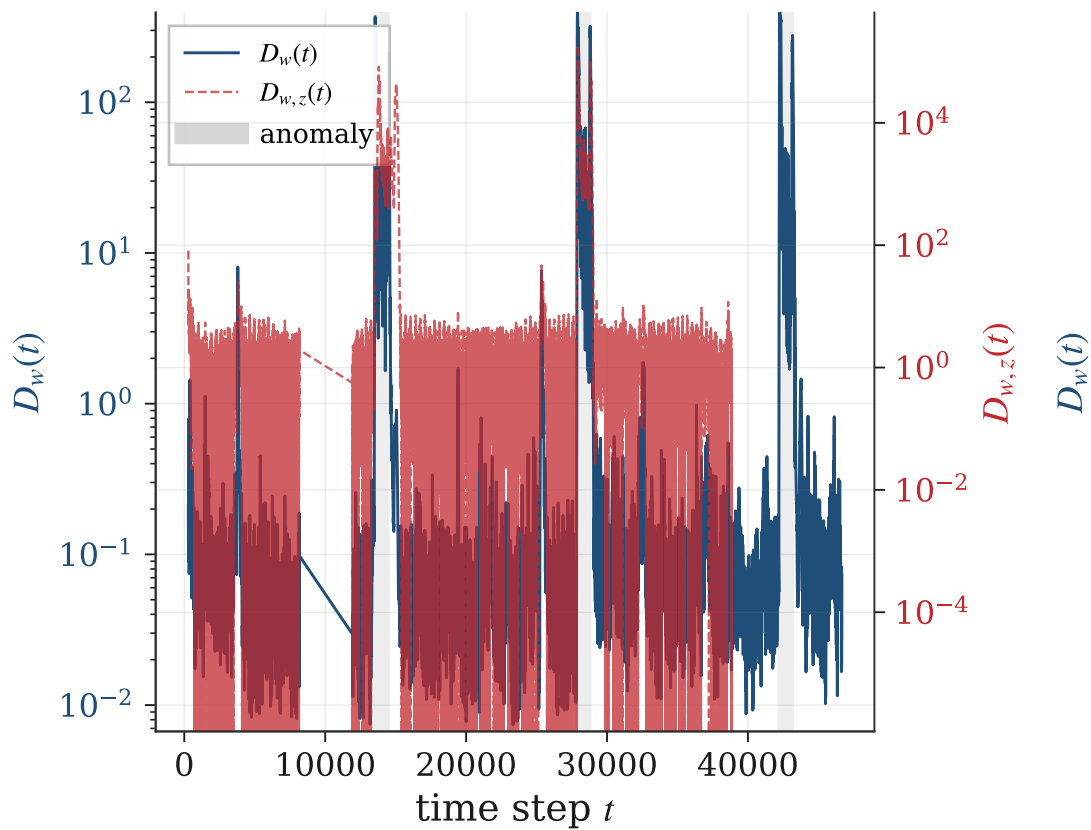
(a) Best: Exathlon_id_16 \text{AUROC}_{D_w} = 0.994 , \text{AUROC}_{D_{w,z}} = 0.978
