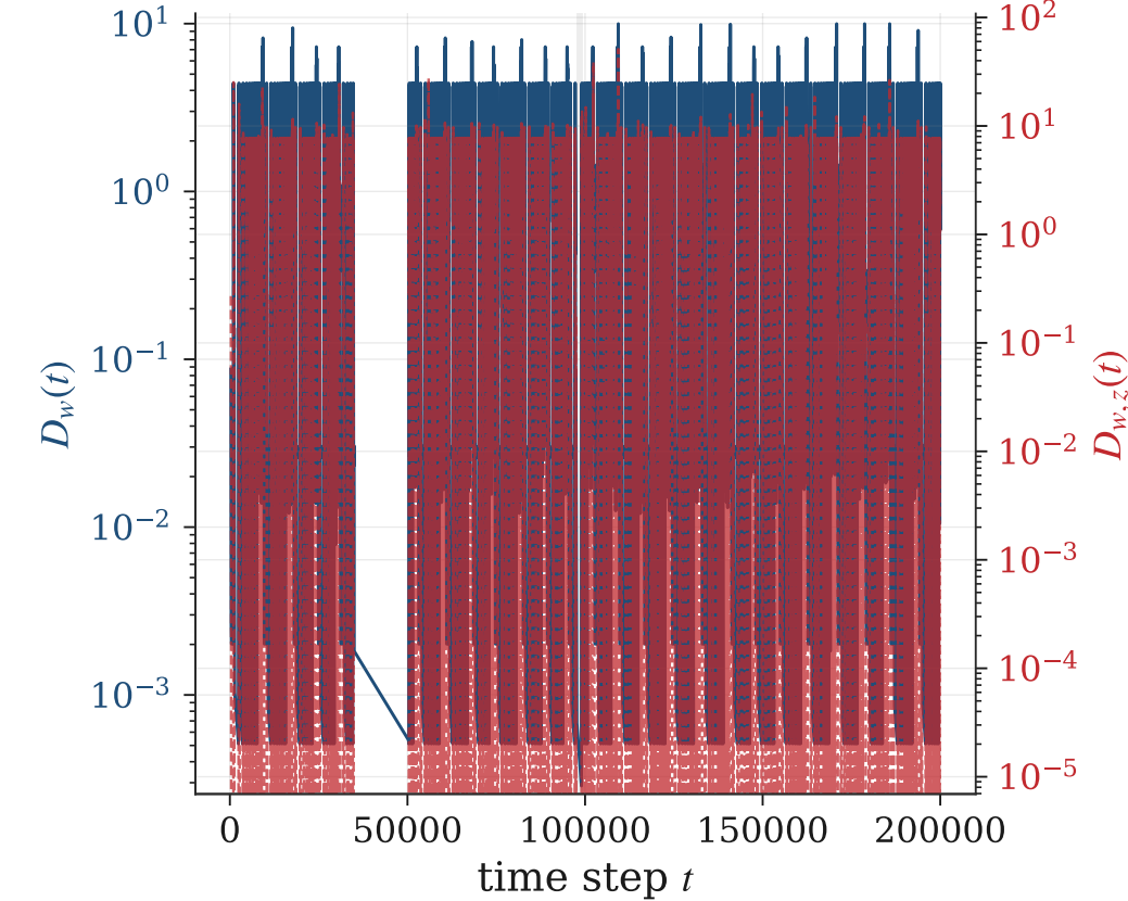
(c) Worst: GHL_id_21 \text{AUROC}_{D_w} = 0.004 , \text{AUROC}_{D_{w,z}} = 0.539
